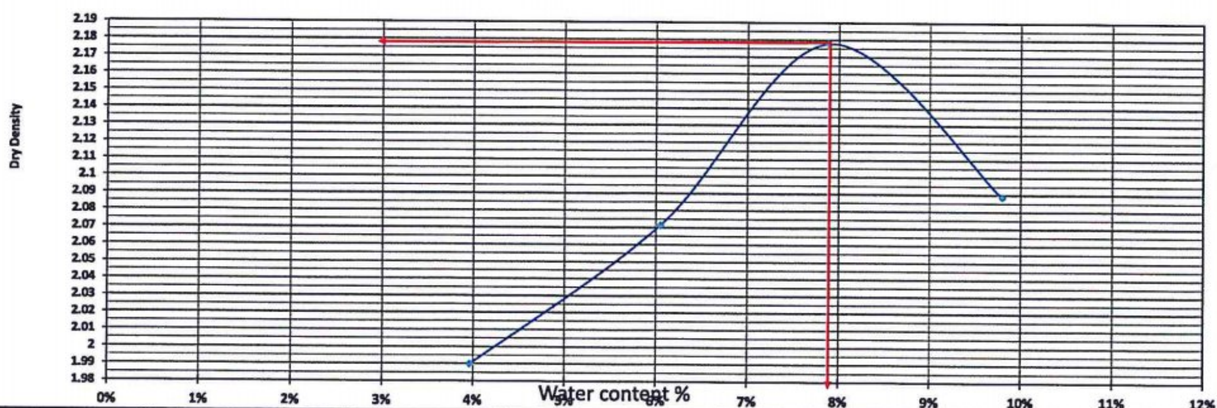
curve proctor
