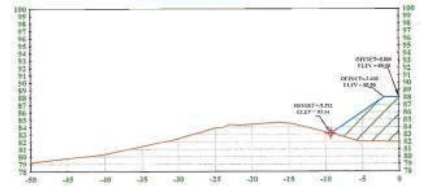
D02 - West Alignment ST:0+250.000
