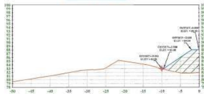
D02 - West Alignment ST:0+245.000
