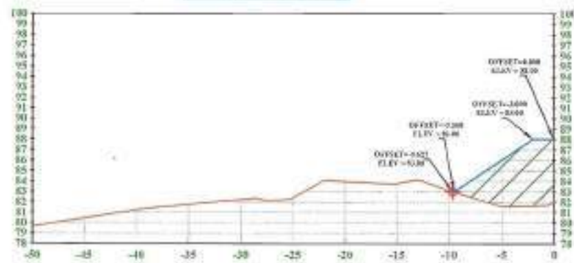
D02 - West Alignment ST:0+240.000
