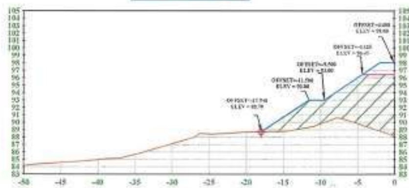
D02 - West Alignment ST:0+105.000
