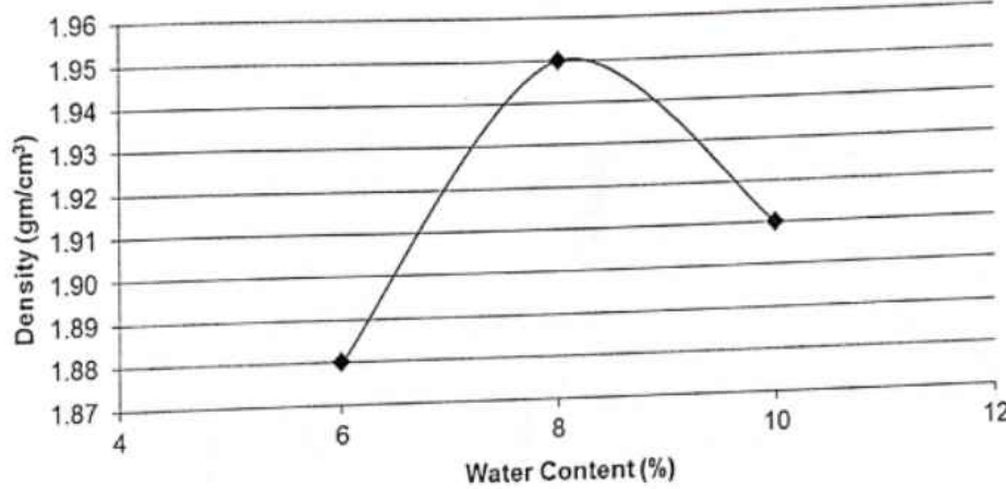
Proctor Test Results
