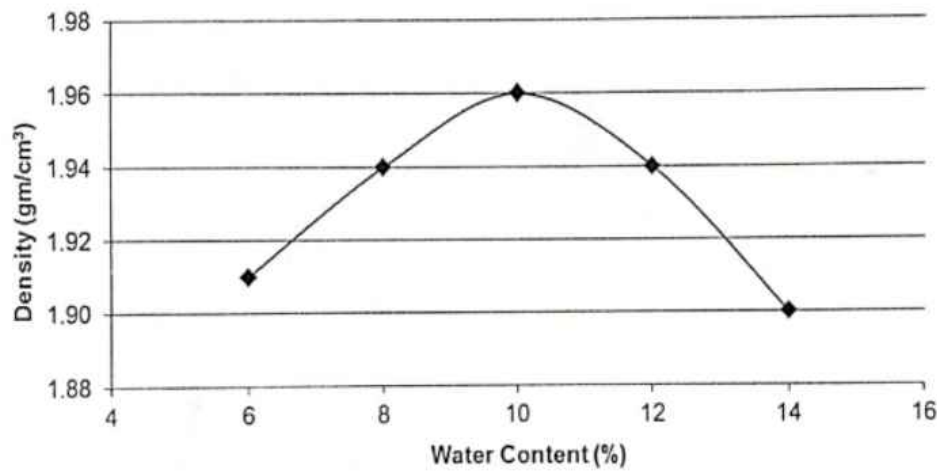
Proctor Test Results
