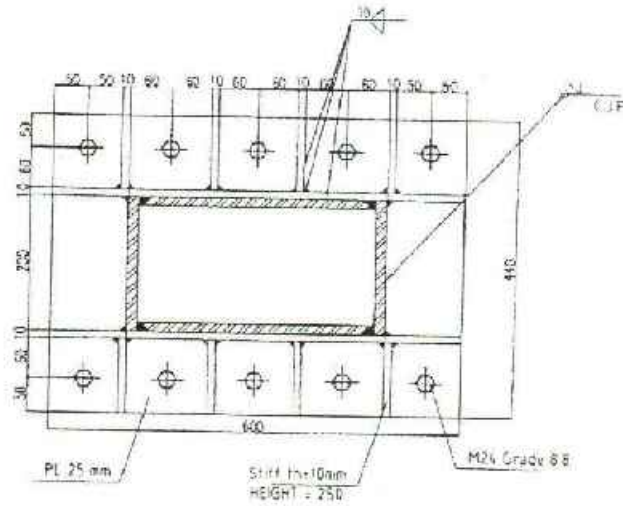
PL1: COLUMN END PLATE
