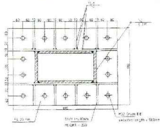
PL3 BASE PLATE
