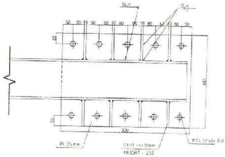
PL2: BEAM PLATE
