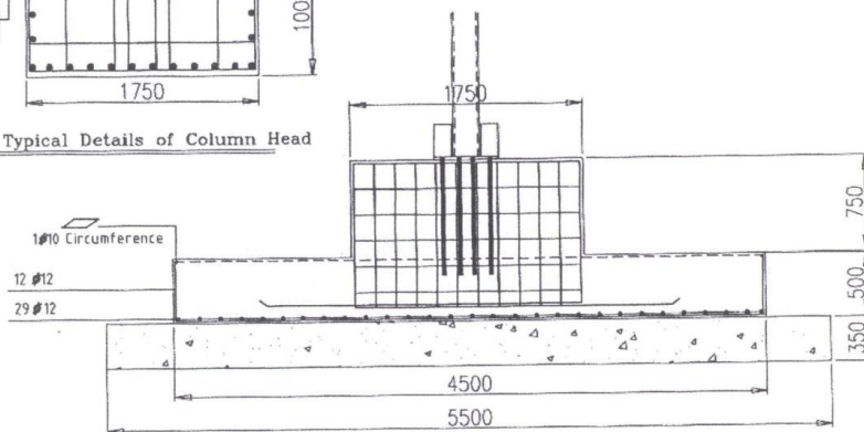
Typical Details for Footings (Parallel with road Direction)
