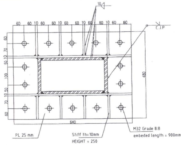
PL3: BASE PLATE
