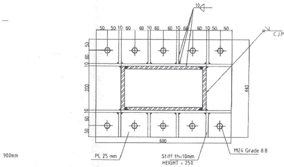
PL1: COLUMN END PLATE
