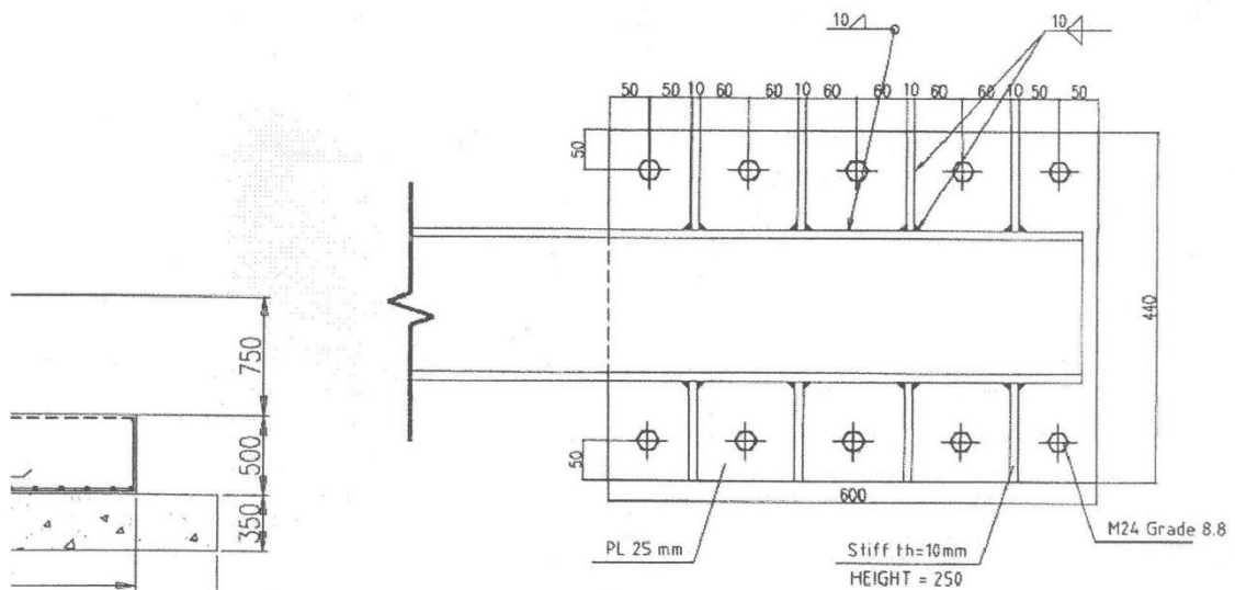
PL2: BEAM PLATE
