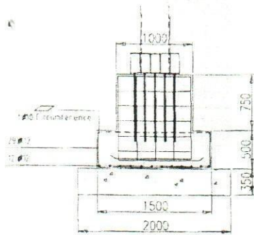
Typical Details for Footings (Perpendicular to road Direction)
