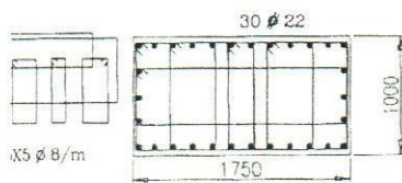
Typical Details of Column Head
