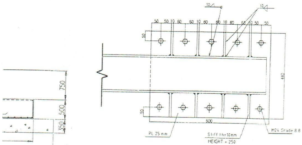
PL2: BEAM PLATE
