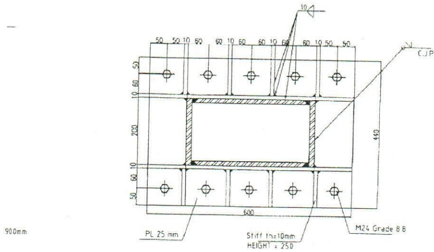
PL1: COLUMN END PLATE
