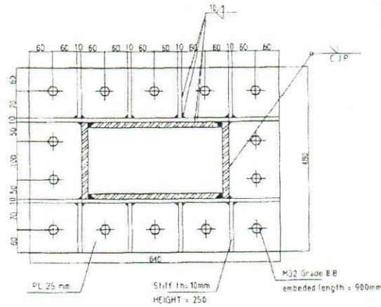
PL3: BASE PLATE
